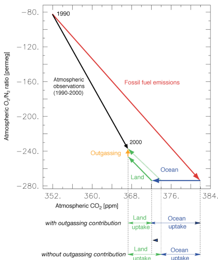
Figure 7: Impact of the oceanic outgassing of oxygen on the atmospheric O 2 /N 2 method for determining the sinks for anthropogenic CO 2 . The diagram shows the observed temporal evolution of the atmospheric O 2 /N 2 ratio versus that of atmospheric CO 2 (black arrow) as well as the different contribution to the global budget for CO 2 and O 2 , i.e. fossil fuel emissions (red arrow), oceanic uptake (blue arrow), land uptake (green arrow), and oceanic outgassing of oxygen (orange arrow). Any uncertainty in the outgassing of oceanic oxygen leads to a nearly corresponding uncertainty in the partitioning of the anthropogenic CO 2 fluxes between the ocean and the land biosphere.
